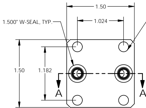
2-PORT
