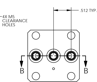
3-PORT, BLIND
