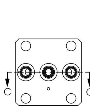
3-PORT, CONNECTED
