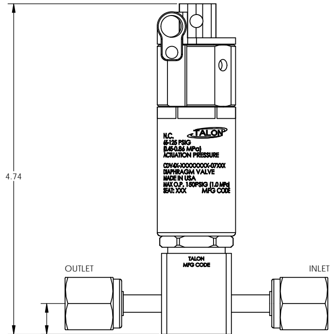
4.74 .44 TYP. OUTLET INLET FEMALE FACE SEAL, SWIVEL A PORT CONFIGURATION TALON MFG CODE
