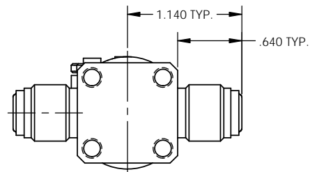
MALE FACE SEAL
