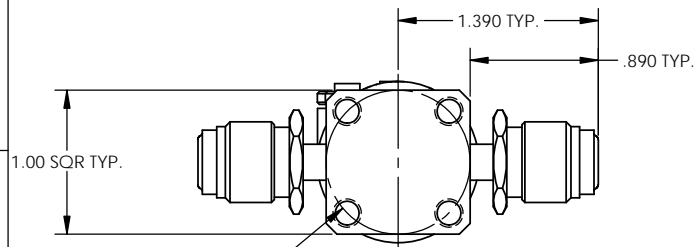
4X M5 X 0.8 EQ SPACE ON Ø1.00 MALE FACE SEAL, SWIVEL
